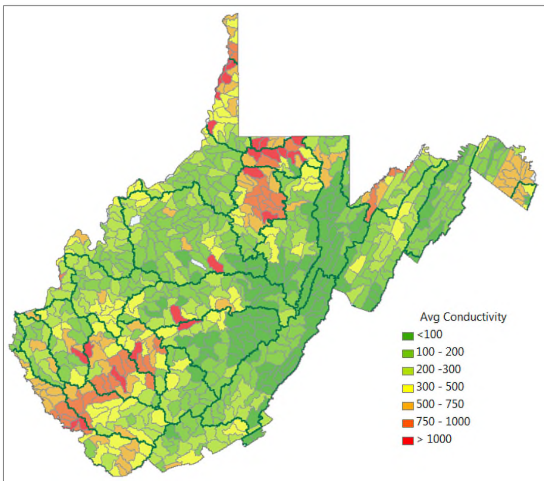
Figure 6: Average Specific Conductance at 12-digit-HUC Scale Watersheds in West Virginia
